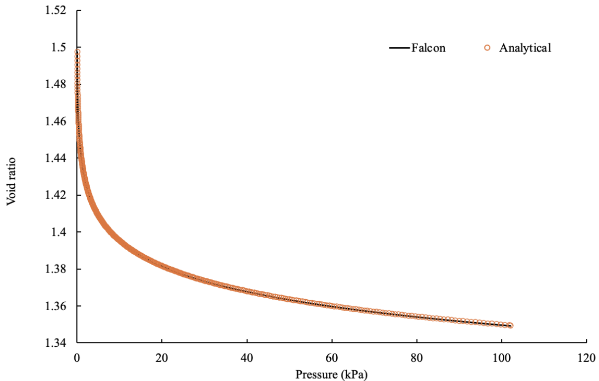
Figure 1: Void ratio vs pressure at (0,10) m
