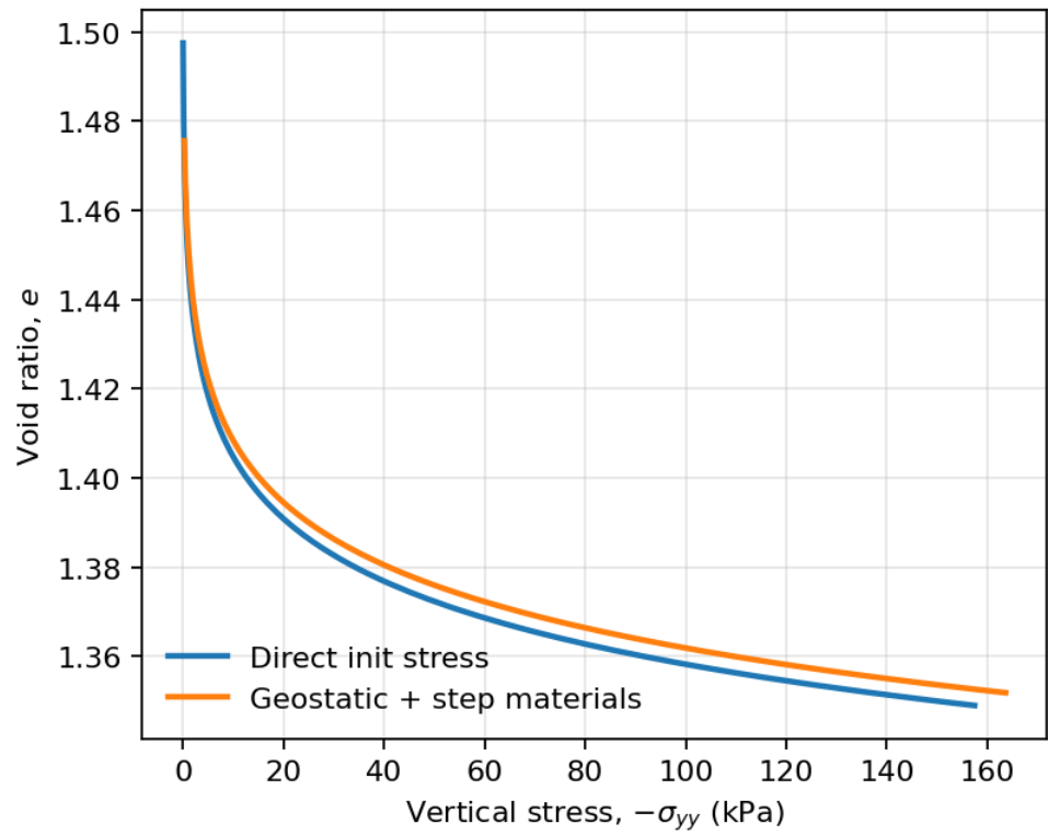
Figure 2: Direct vs step-materials comparison
